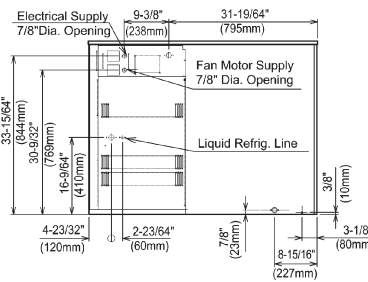
KM-2400SRH3 REMOTE AIR-COOLED UNIT
