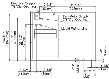
KM-2000SRH3 REMOTE AIR-COOLED UNIT
