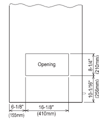
ICE DROP ZONE - KM-2000/2400
